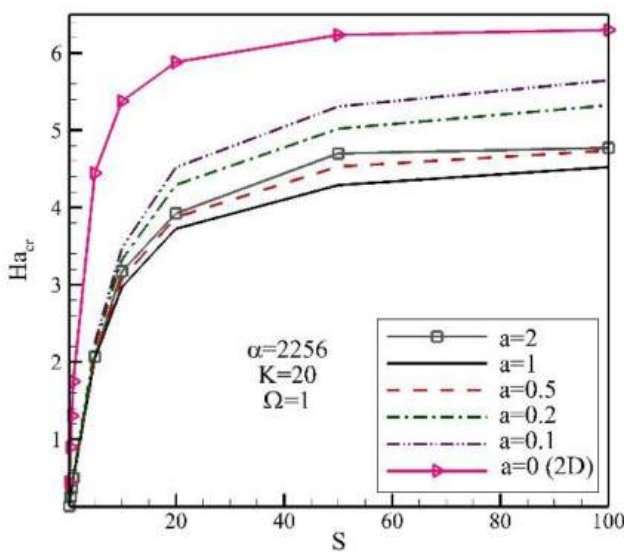
Figure 13. Critical Hartmann number by means of dimensionless lateral electric field under influence of \alpha = 2256 , K = 20 , and \Omega = 1 in different values of aspect ratio.
