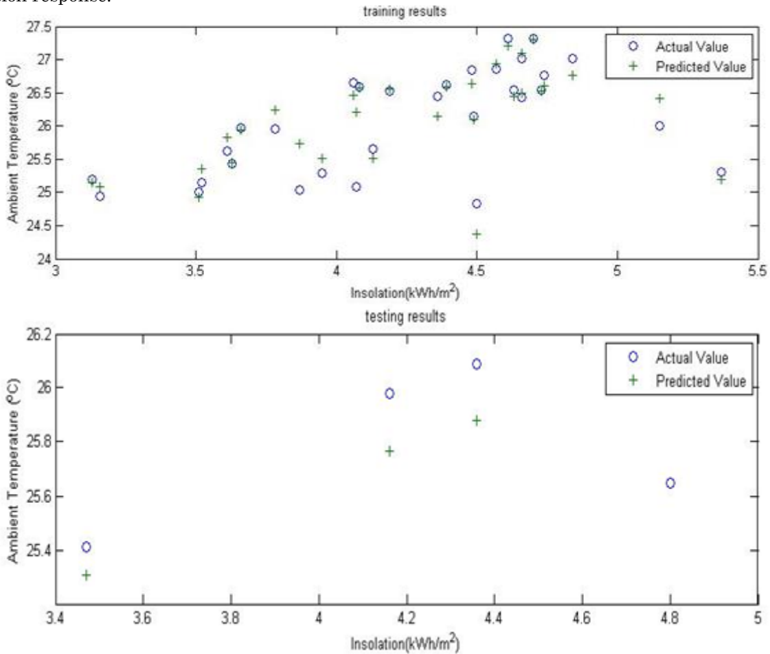
Fig.2. Neural Prediction Response (90% Training data)
